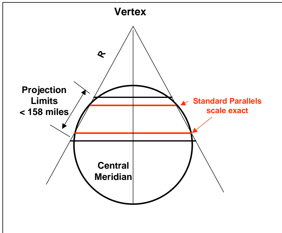
Figure 5-7. Lambert Projection
