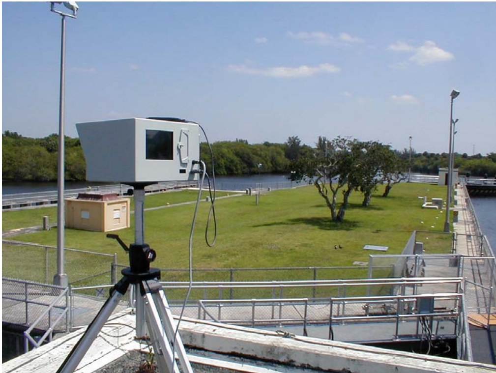
Figure 10-1. Optech ILRIS 3D laser scanner--detailed mapping of structures and facilities at St. Lucie Lock and Dam, Jacksonville District (Arc Surveying & Mapping, Inc.)
