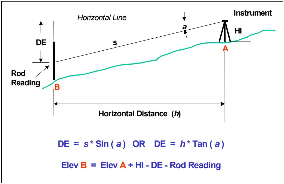
Figure 3-14. Trigonometric leveling
