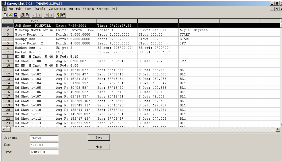
Figure 11-7. Editing total station raw data file in TDS Survey Link 7.03
