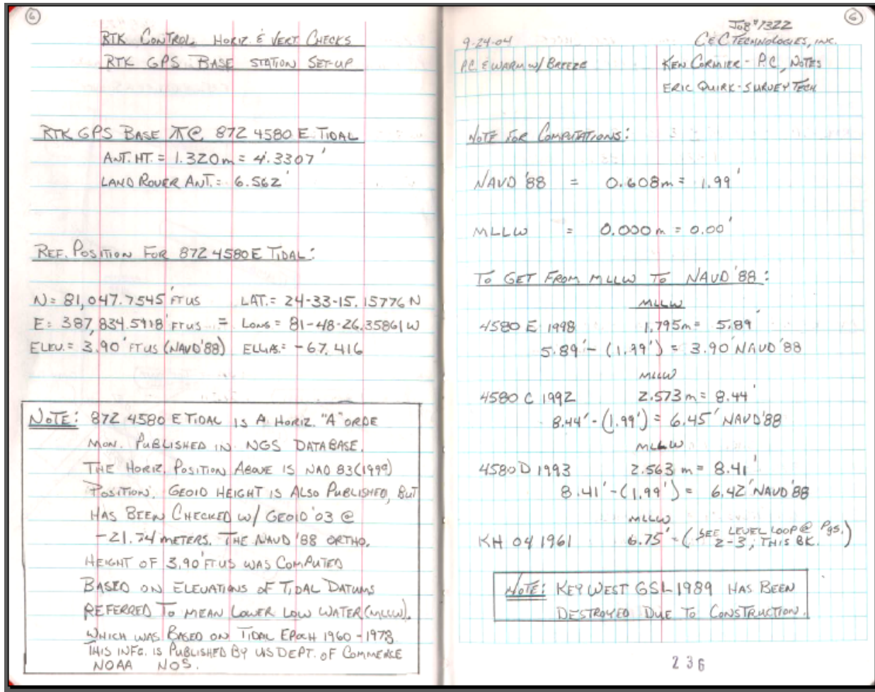
Figure 12-3. RTK reference notes in a field survey book (Jacksonville District--C&C Technologies, Inc.)
